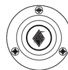
FRONT FLUSH MOUNT VIEW USING MOUNTING SCREWS FROM FRONT
